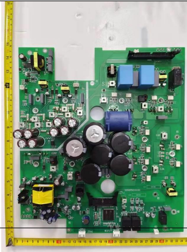
Internal view-
