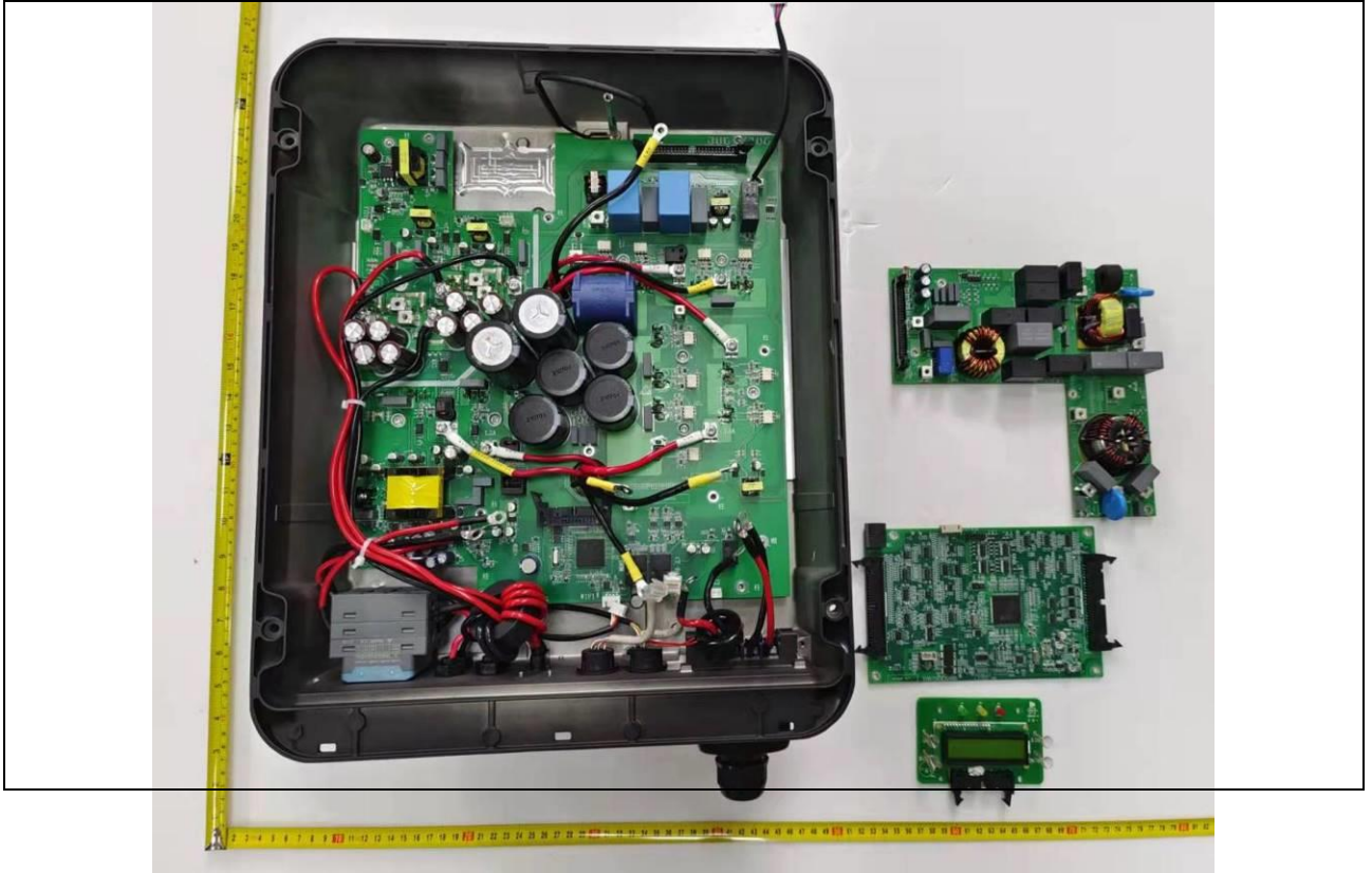
Internal view-
